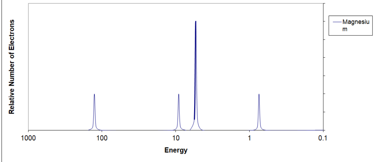
Photo Electron Spectra
