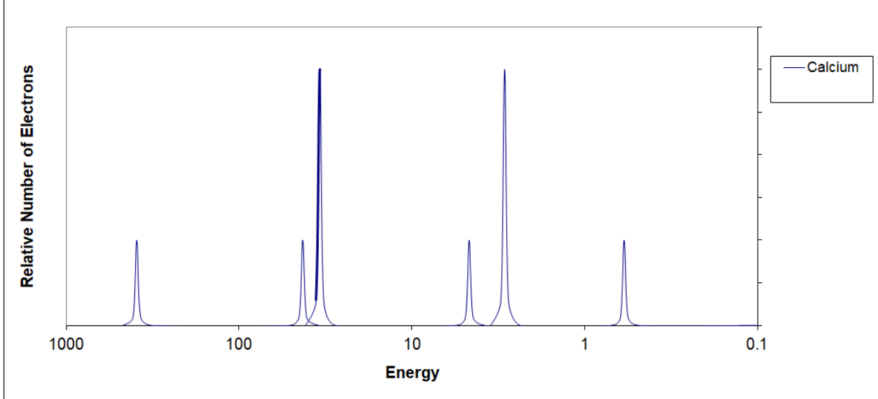
Photo Electron Spectra
